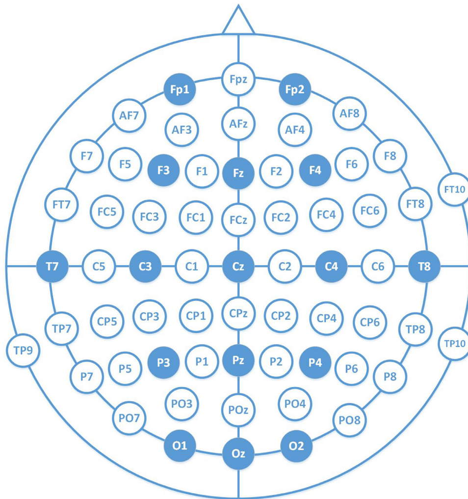
Figure 2. Electrodes placement.
