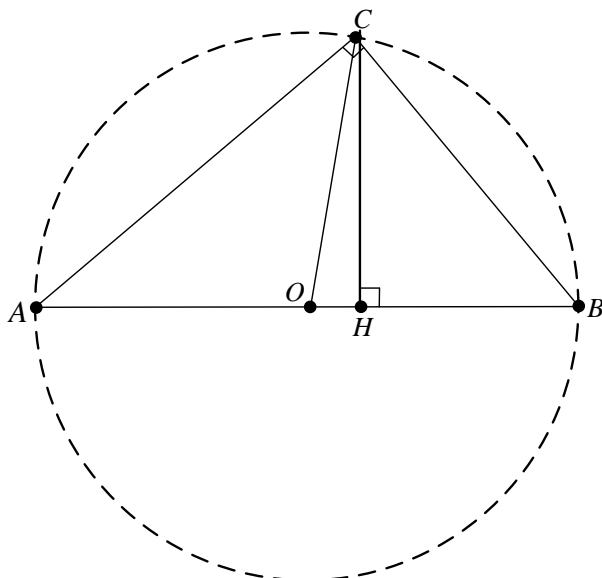
Figure 2. A triangle in a circle with a symmedian Source: developed by the author
